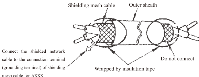
Wrapping end of shielded twisted pair cable
