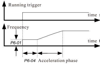
Start frequency figure
