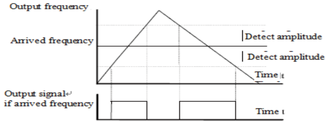
The function of arrived frequency detect figure
