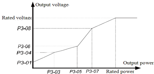
Multistage V/F curve figure:
