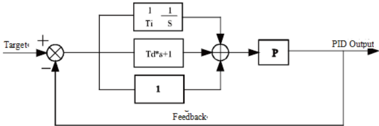
PID Control figure
