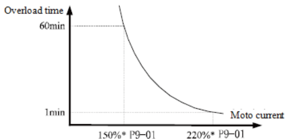
Moto overload curve
