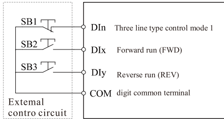
Three line type control mode 1
