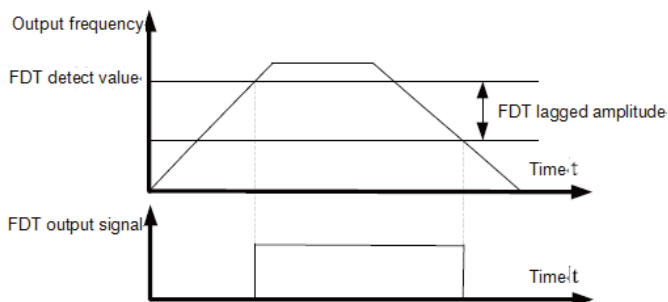
FDT signal figure
