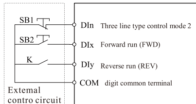
Three line type control mode 2
