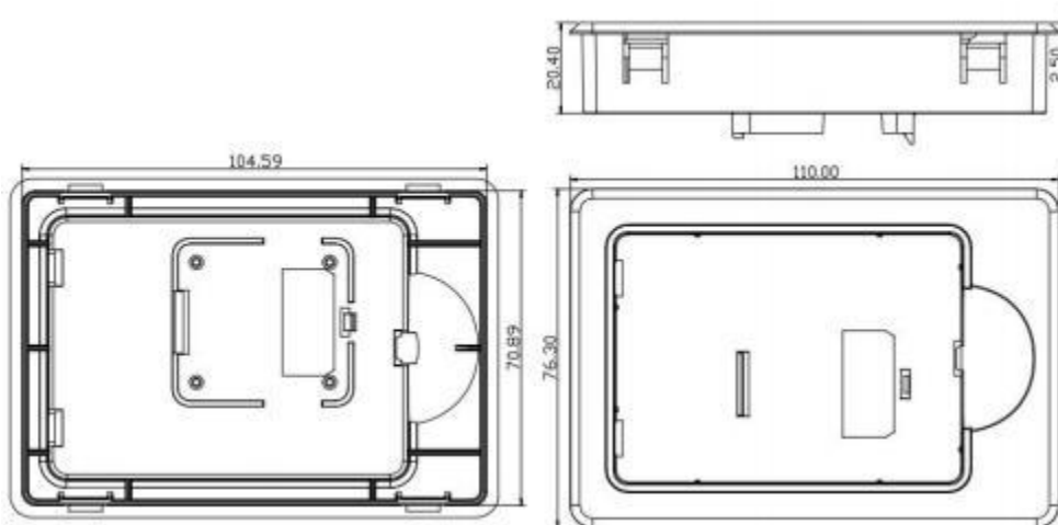
迷你型面板尺寸图*
